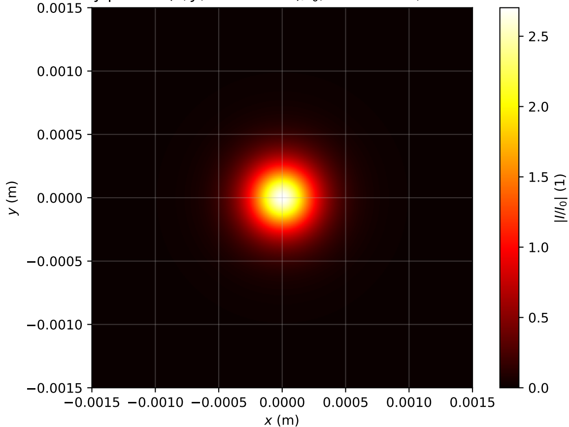
Intensity profile I(x, y, z = 3.105m)/I_0 , Pin=1.0Pcr, artificial time
